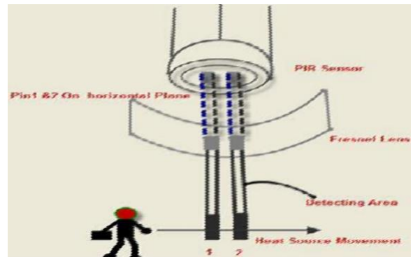
Figure 1.2: PIR Sensor.
