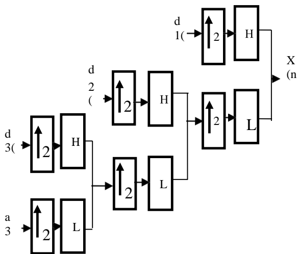
Figure 2 Wavelet Reconstruction
