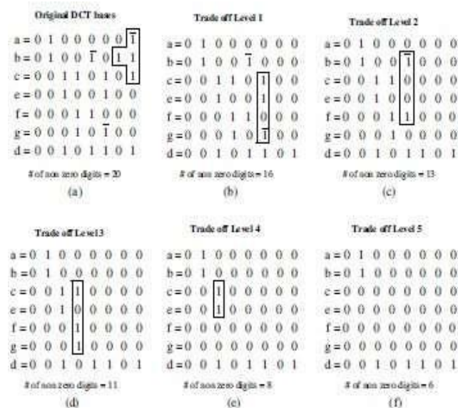
Fig. 3: Constant multiplier Approximation
