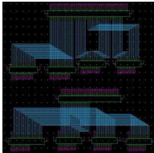
Fig. 7: Proposed energy efficient approximate DCT architecture on Tanner
