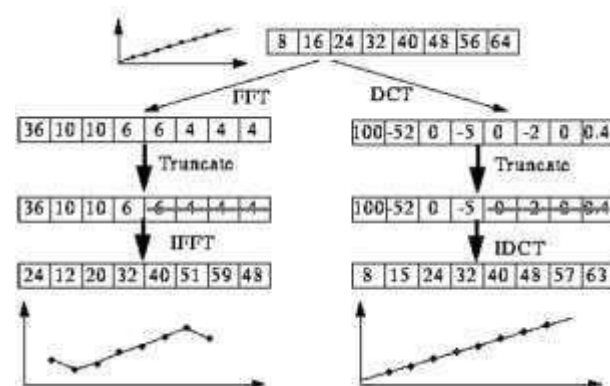
Fig. 2: Illustration of energy compaction property.
