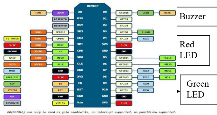
Fig 1 Pin definition
